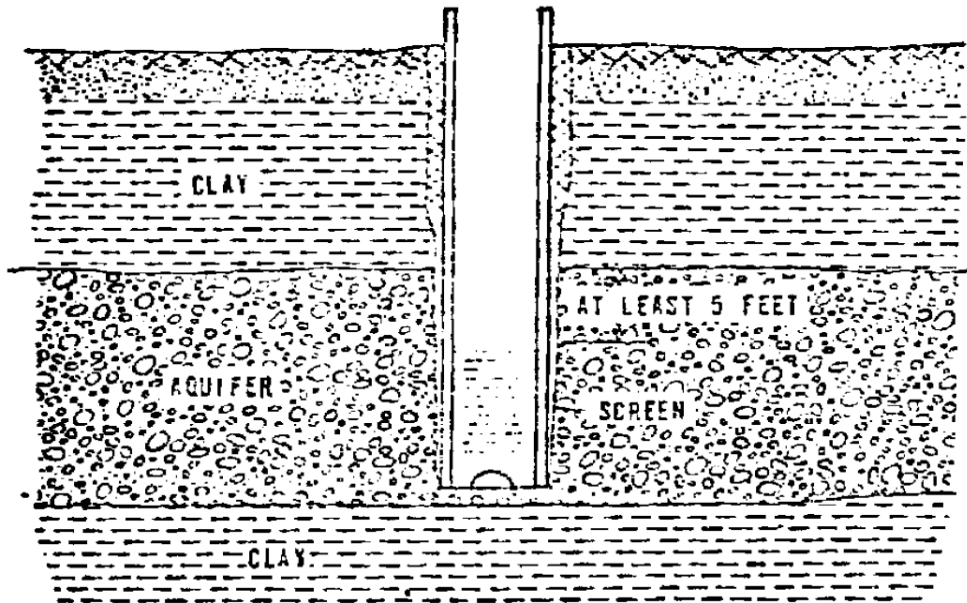
FIG. 5 CONSTRUCTION OF WELL IN AOUIFER OVERLAIN BY CLAY
